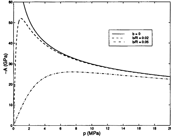
Fig. 2. Path independent ema for one of the 3rd order elastic constants of frictionless glass beads, as a function of confining pressure.
