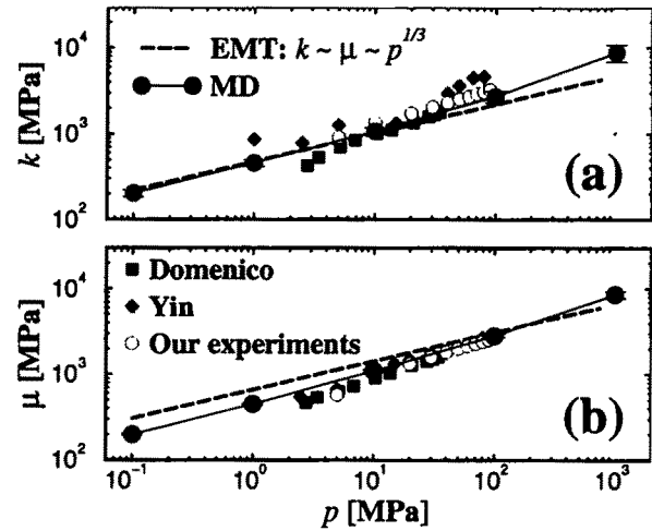
Fig. 4. Pressure dependence of the elastic moduli from molecular dynamics simulations, experiments, and path dependent ema : (a) bulk modulus, and (b) shear modulus. The data are from Domenico (1977), Yin (1993), and Makse, et al. (1999).
