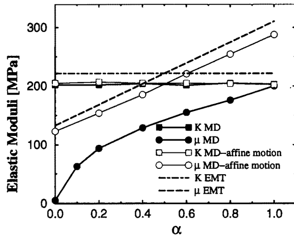
Fig. 5. Bulk modulus, K , and shear modulus, \mu , vs. \alpha for a fixed pressure, p=100\text{kPa} . The effective medium theory is compared against the unrestricted numerical simulations. For comparison, we also show the results of simulations in which the displacement of each grain is restricted to affine motion and rotation is disallowed.
