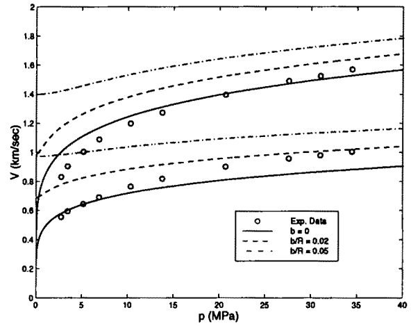
Fig. 1. Path independent ema predictions of pressure dependent sound speeds of granular media with welded contacts. The upper three curves and the upper data set refer to compressional wave speeds, whereas the lower curves and data set refer to transverse wave speeds. The experimental data of Domenico (1977) should be compared against the b = 0 curves. A coordination number Z = 9 was assumed. From Norris and Johnson (1997).
